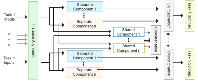
Fig. 2. Structural multi-task learning for psychometric dimensions
