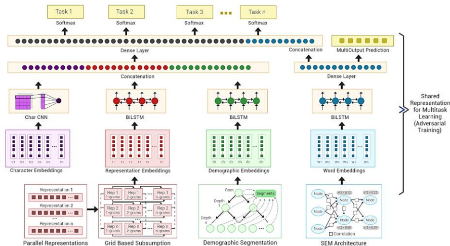
Fig. 1. PyNDA - proposed psychometric NLP deep learning architecture.
